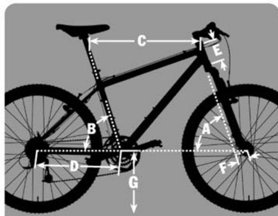
A Head Tube Angle B Seat Tube Angle C Top Tube Length D Chain Stay Length E Head Tube Length F Fork Offset G Bottom Bracket Height
